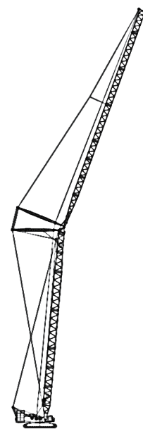
Standard tower jib working condition (HW)
