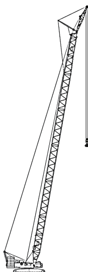
Standard fixed jib working condition (HF)
