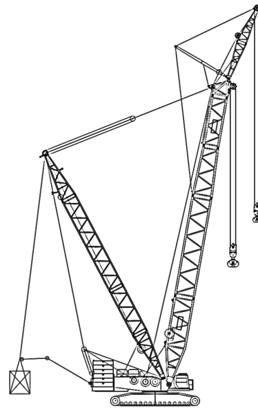
Superlift TBM working condition (SHFS)
